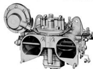
Type 44 PHH (Horizontal) Carburetor
