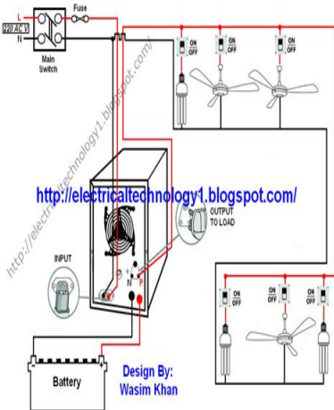
Automatic UPS system wiring diagram for Home or Office (New Design with One Live wire)
